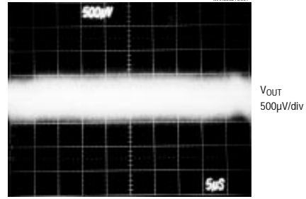
OUT2 NOISE AND RIPPLE
